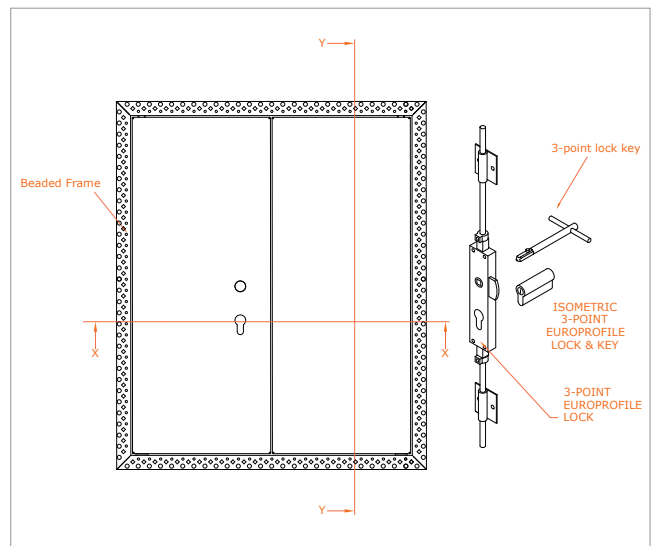
Non-fire rated, beaded frame, 3 point high security locking, double door
