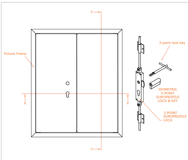
Non-fire rated, picture frame, 3 point high security locking, double door
